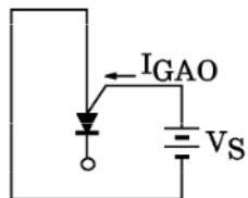
Fig.4 IGAO test circuit
