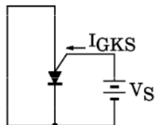
Fig.5 IGKS test circuit
