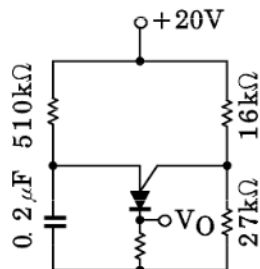
Fig.6 V O and t r test circuit
