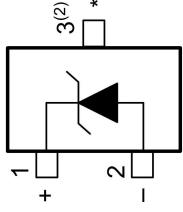
Figure 4-1. DBZ Package 3-Pin SOT-23 Top View
