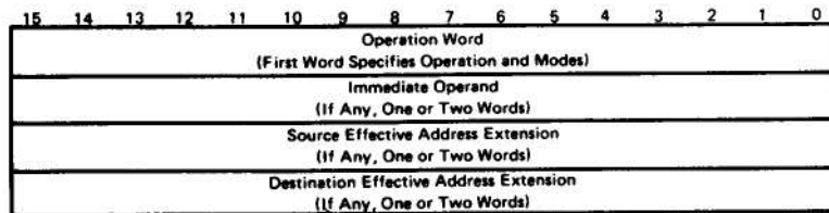
Figure 12 Instruction Format
