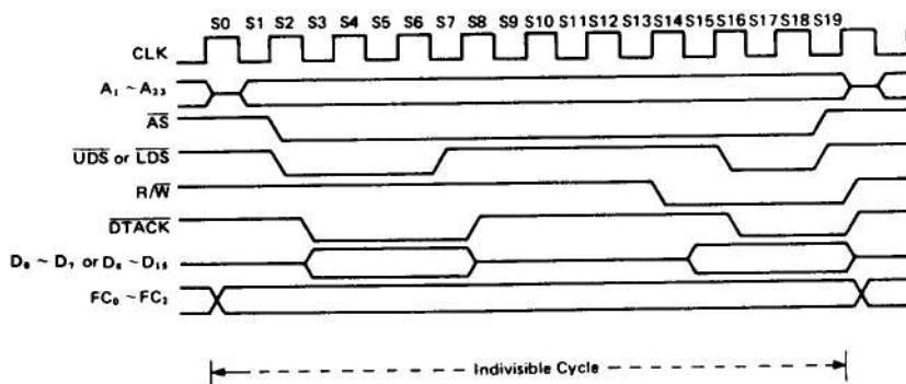
Figure 23 Read-Modify-Write Cycle Timing Diagram
