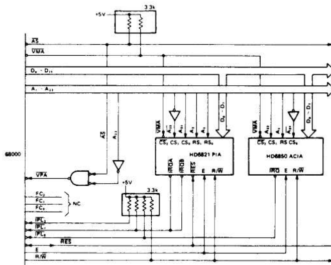
Figure 52 HD6800 Interface—Example 1
