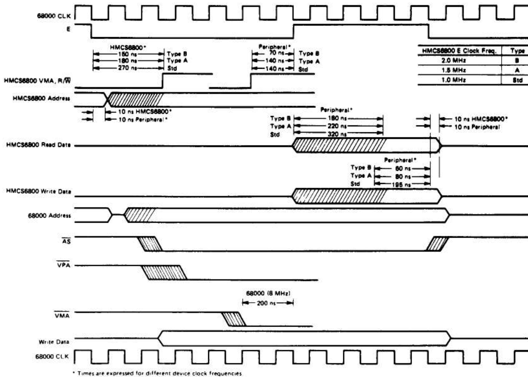
Figure 51 68000 to HD6800 Peripheral Timing Diagram
