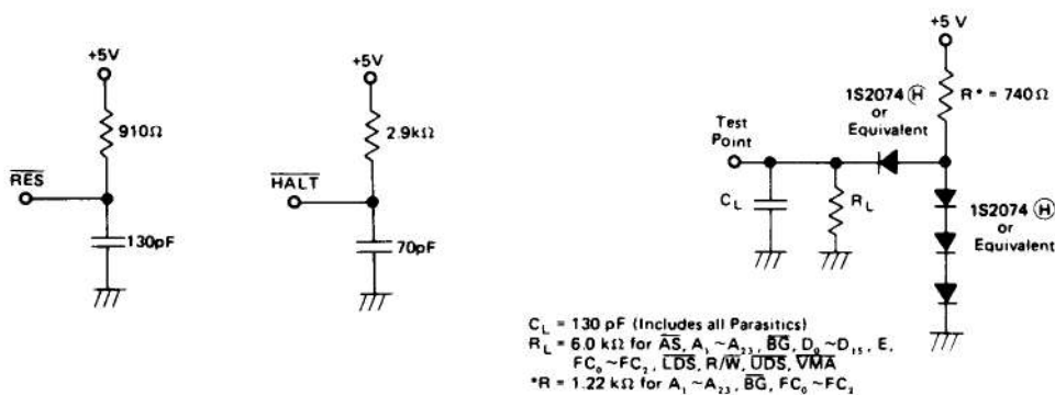
Figure 1 Test Loads
