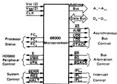
Figure 14 Input and Output Signals
