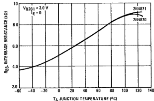
FIGURE 11 — EFFECT OF TEMPERATURE
