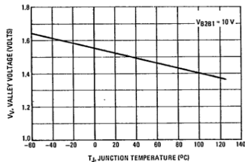
FIGURE 15 — EFFECT OF TEMPERATURE
