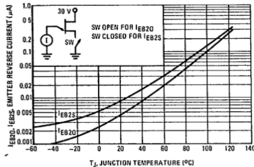
FIGURE 6 — EMITTER REVERSE CURRENT
