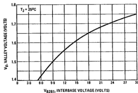
FIGURE 14 — EFFECT OF VOLTAGE
