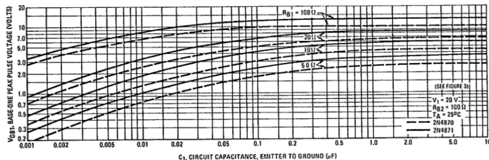
FIGURE 16 — OUTPUT VOLTAGE
