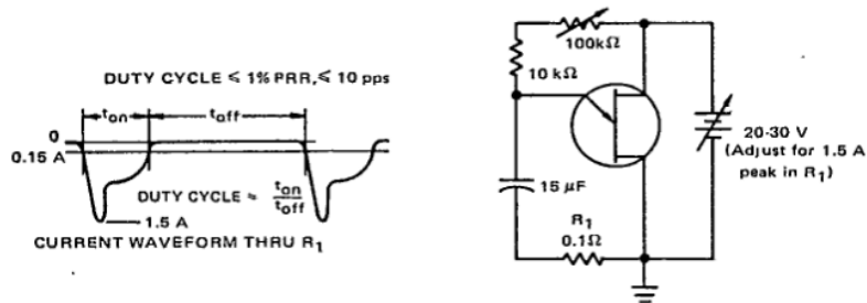
FIGURE 5 — PRR TEST CIRCUIT AND WAVEFORM
