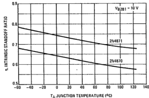
FIGURE 7 — INTRINSIC STANDOFF RATIO
