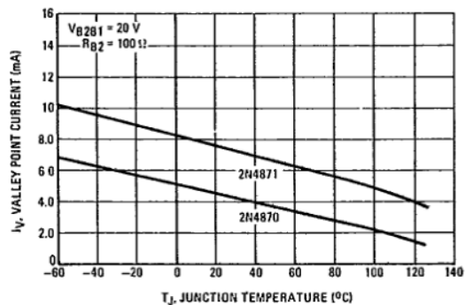
FIGURE 13 — EFFECT OF TEMPERATURE
