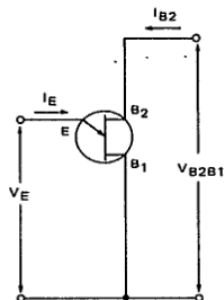
FIGURE 1 — UNIJUNCTION TRANSISTOR SYMBOL AND NOMENCLATURE
