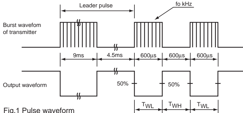
Fig.1 Pulse waveform
