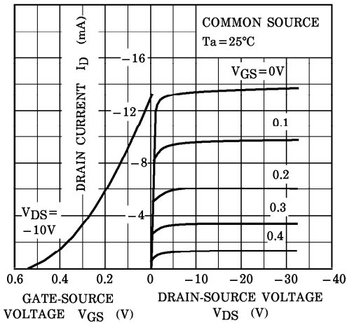
STATIC CHARACTERISTICS
